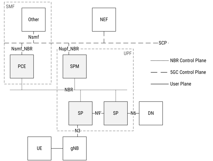
Fig. 3. Modified System Architecture for Name-Based Routing - Infrastructure Mode.
