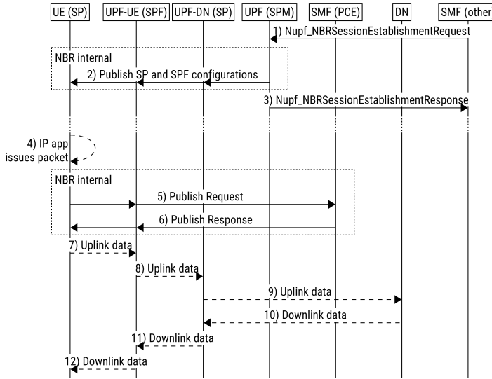
Fig. 8. Session Establishment for Name-Based Routing-Based User Plane Functions Operating in UE Mode.
