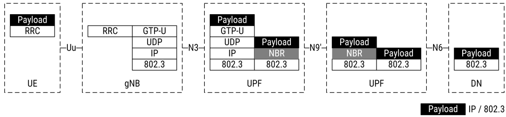
Fig. 4. Name-Based Routing user plane protocol stack for infrastructure mode for both Packet Data Unit session types IP and 802.3.
