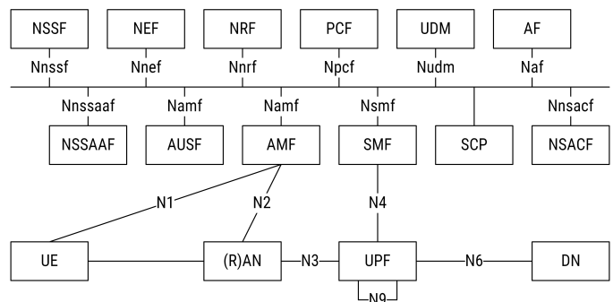
Fig. 1. 3GPP’s 5G System Architecture [1]
