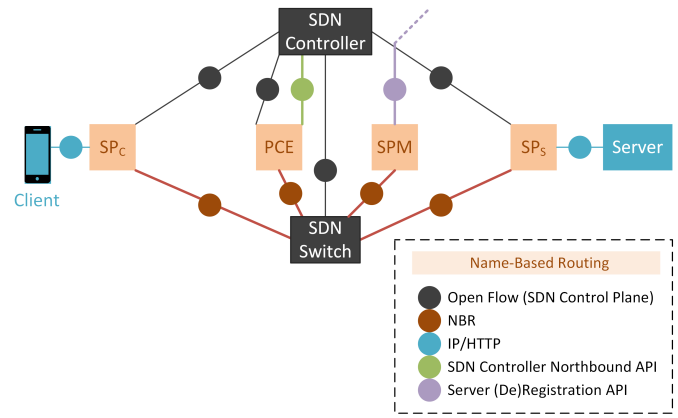
Fig. 2. Internal Architecture of Name-Based Routing with Software-Defined Networks Integration.
