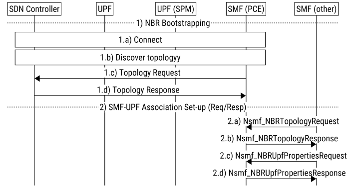
Fig. 9. SDN-Based Session Management Function and User Plane Function Provisioning.
