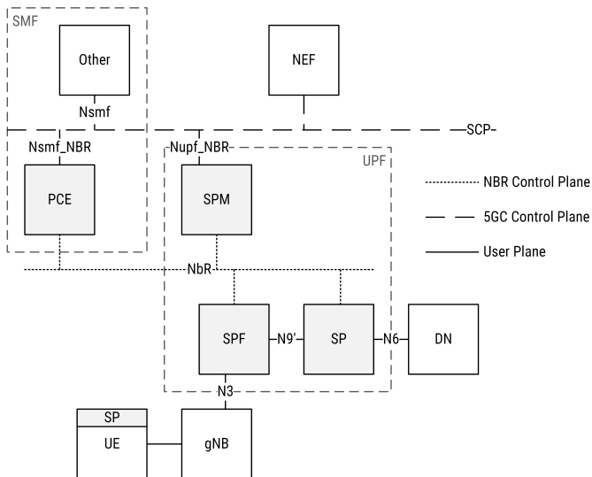
Fig. 6. Modified System Architecture for Name-Based Routing - User Equipment Mode.
