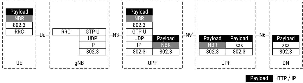
Fig. 7. Protocol Stack for 5G User Plane in Name-Based Routing UE mode.
