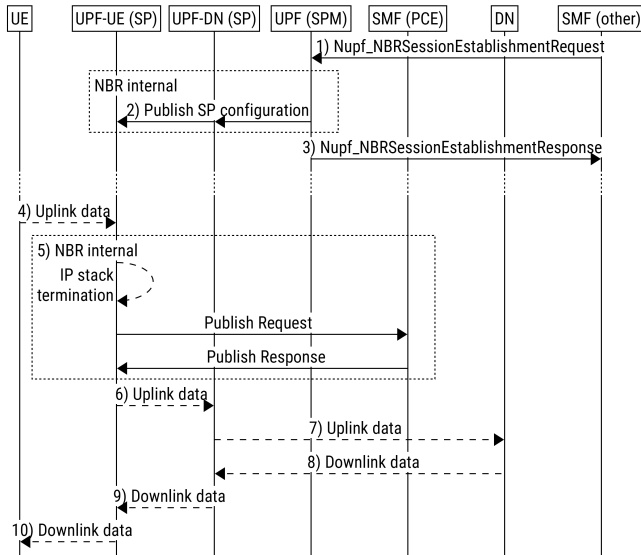
Fig. 5. Session Establishment for NBR-based UPFs Operating in UE Mode.
